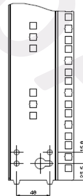
DETAIL OF 19" UPRIGHT
