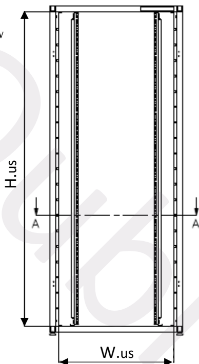
Front view
